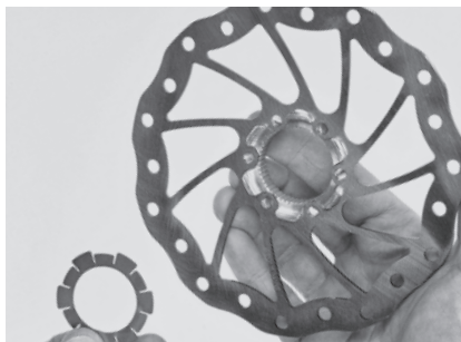
1. The lock washer is mounted after the adaptor has been stuck on the SL-rotor.
